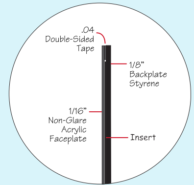
Section View
